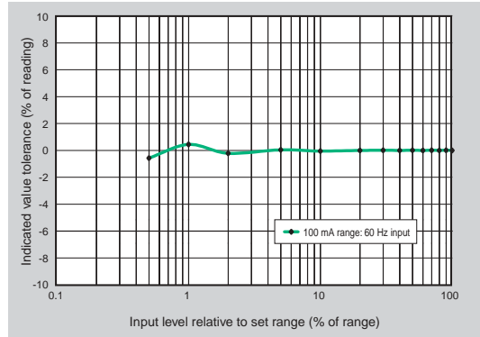
Example of WT210 Current Accuracy
